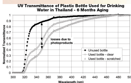
Figure 14b: The UV-transmittance losses due to photoproducts
