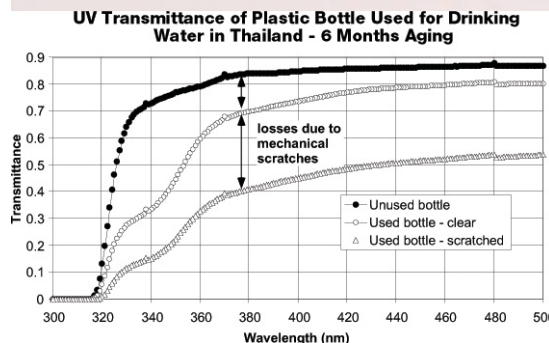
Figure 14a: The UV-transmittance losses due to mechanical scratches
