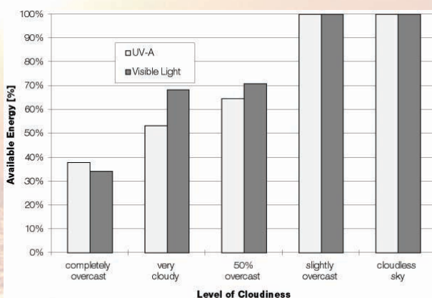
Figure 10: Losses of available solar energy at different weather conditions [16]
